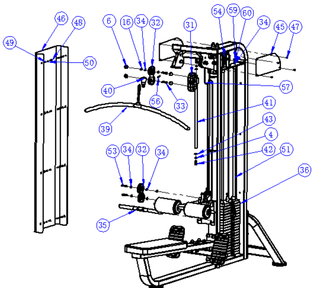
6) Step 6 Pulley installation instruction:
