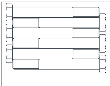
#7 M12*105 × 6PCS
