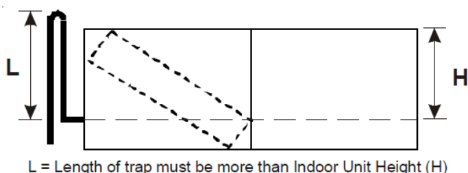
Figure 4-1 Indoor Unit with Inverted Suction
