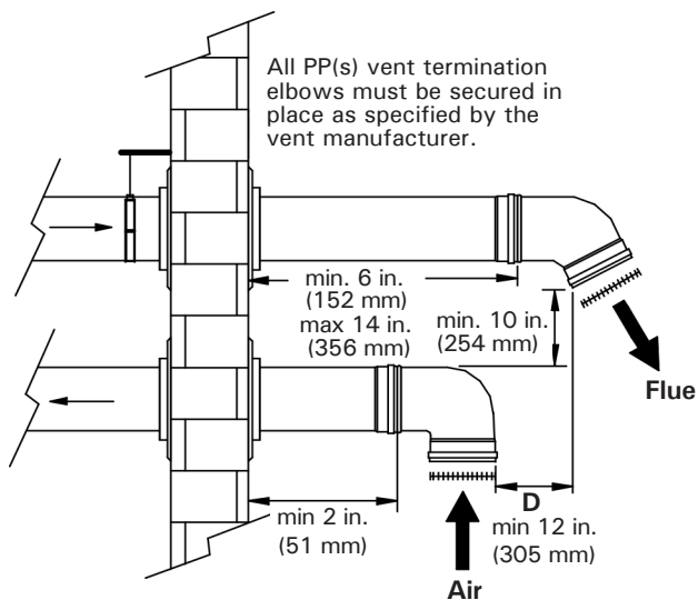
Side wall vent termination (side view)
