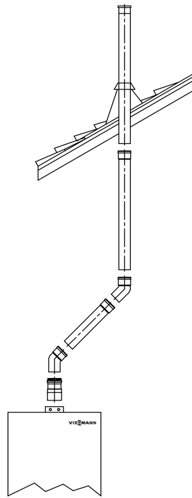
Sloped roof installation with offset
