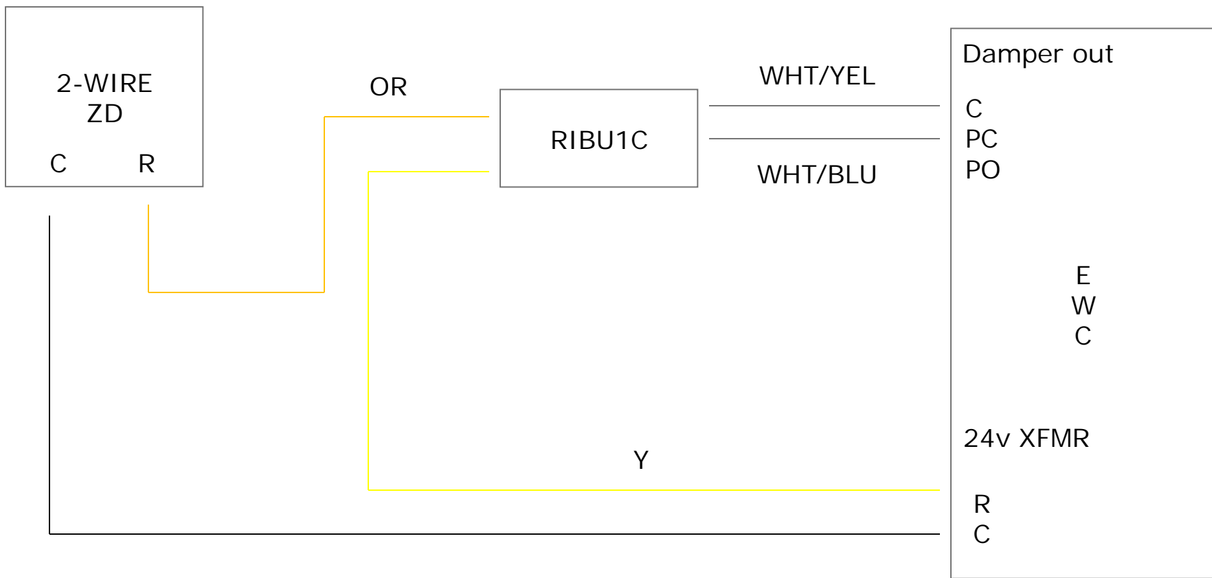
FOR DAMPER MOTORS 2.4VA AND ABOVE
