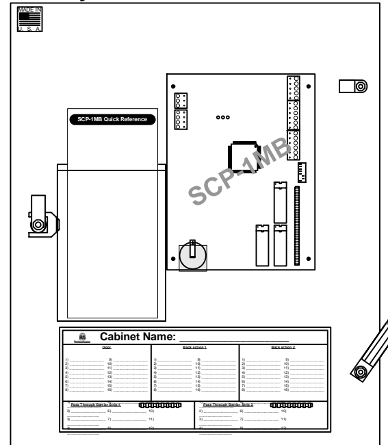
Inside door with a SCP-1MB mounted to it.
