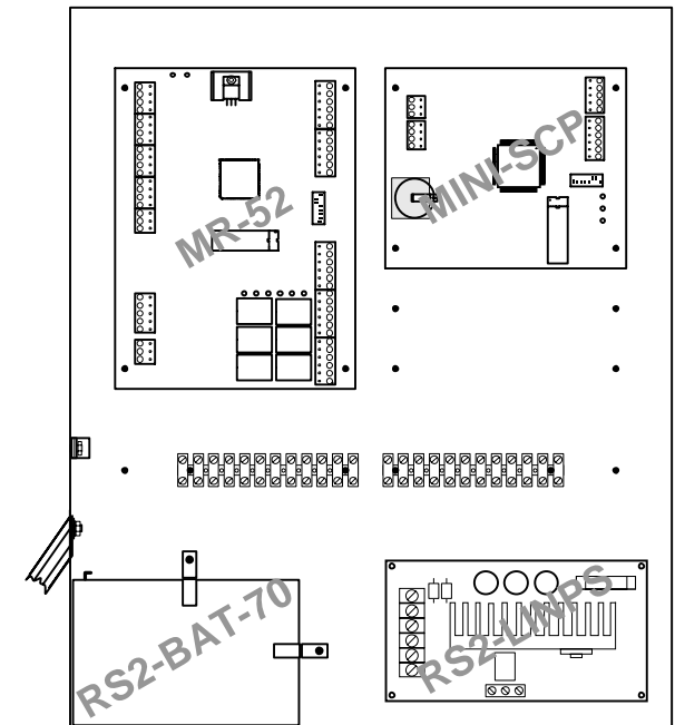
The inside cabinet with a MR-52 and a MINI-SCP mounted in an auxiliary position. Shown with both the optional RS2-LINPS linear power supply and the optional RS2-BAT-70 battery backup kit.
