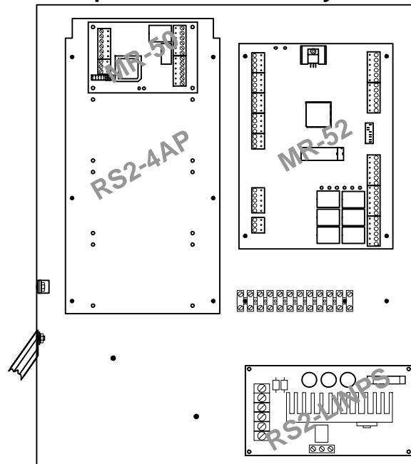
The inside cabinet with a MR-50 mounted on a RS2-4AP and a MR-52. Shown with the optional RS2-LINPS linear power supply.
