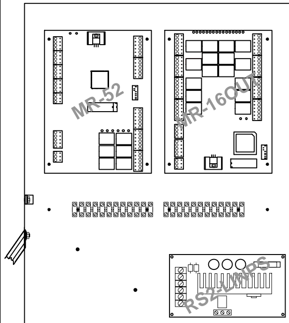
Typical inside cabinet installation with a MR-52 and MR-16OUT mounted within it. Shown with the optional RS2-LINPS linear power supply.
